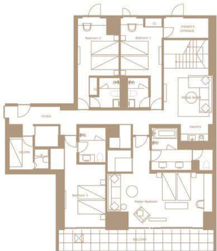
LOWER FLOOR
